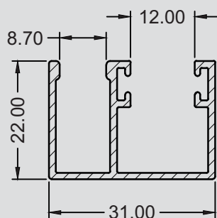
SP-0161 0.383 KG/M
